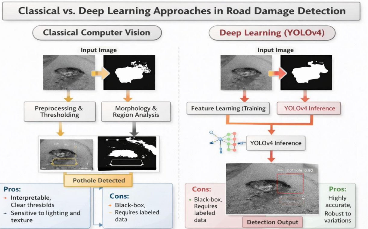
Figure 2.1: Overview of Classical vs. Deep Learning Approaches in Road Damage Detection
